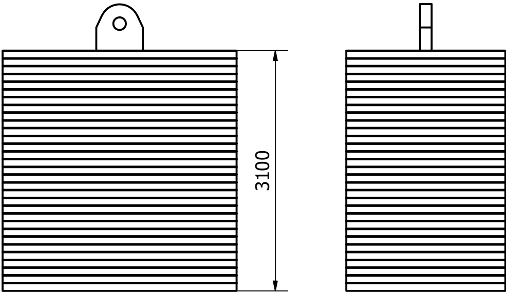
DMA with all additional 28 plates - Maximum size Base + 28 plates
