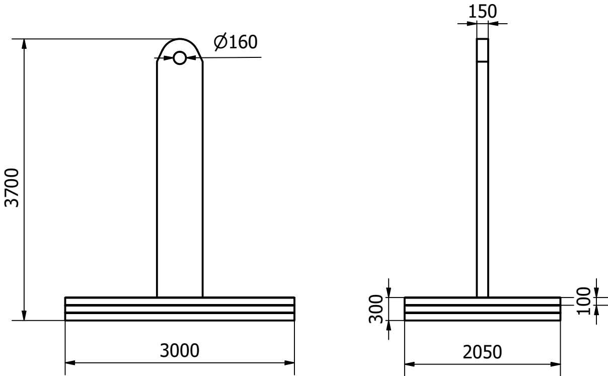
DMA Base - Minimum size Consists of 3 plates fixed to a center pole
